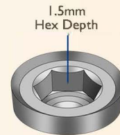
4.5mmD Platform with a 2.5mmD Internal Hex
